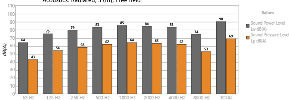
Acoustics: Radiated, 3 (m), Free field
